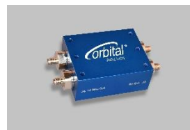
Bias Tee with L Band and 10MHz Pass-Through
